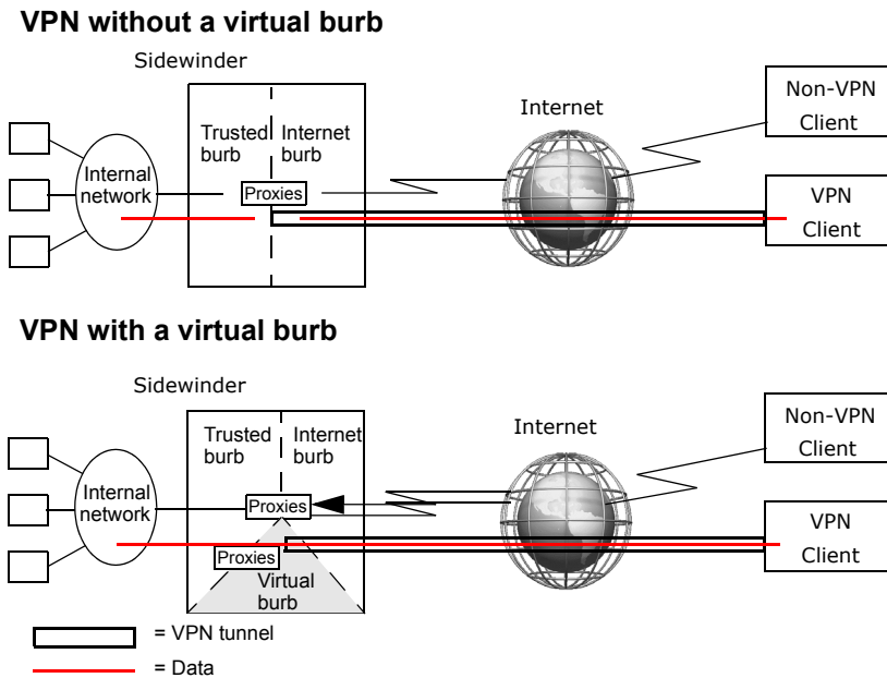
Figure 309 Virtual burb vs. a non-virtual burb VPN implementation
