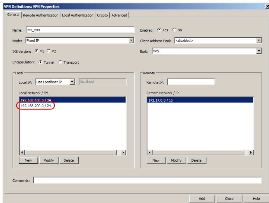
Figure 314 Matching your security policy with your NAT policy
