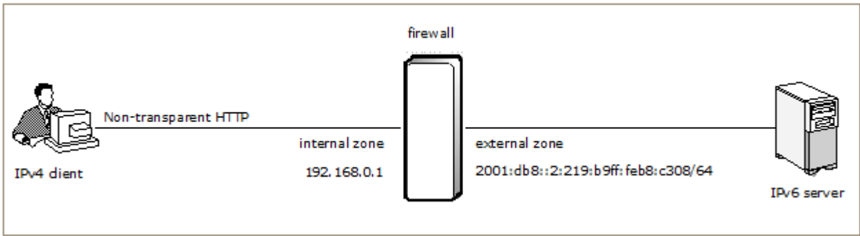
Figure 17: IPv4-to-IPv6 translation
