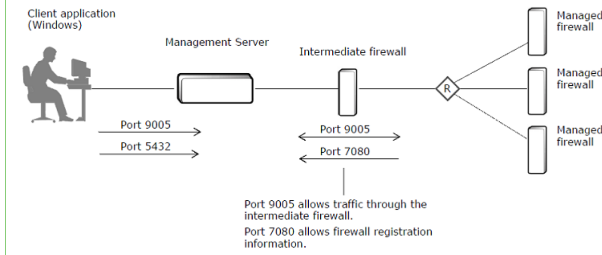
Figure 32: Management Server environment with an intermediate firewall
