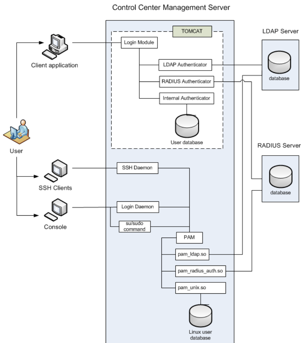
Figure 27: Authentication for the Control Center user
