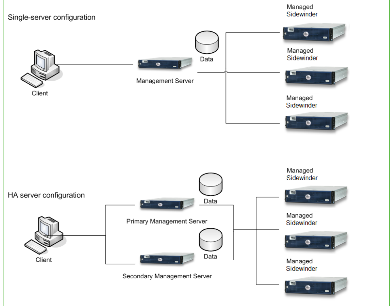
Figure 29: High Availability Management Server configuration
