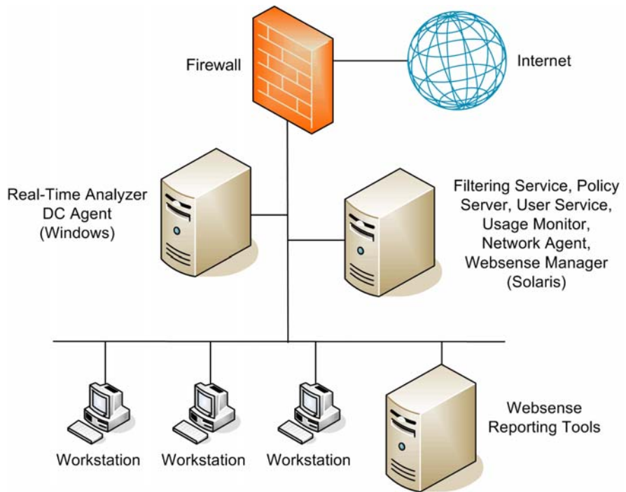
Stand-Alone Deployment in a Solaris Environment
