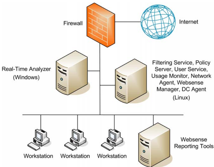
Stand-Alone Deployment in a Linux Environment
