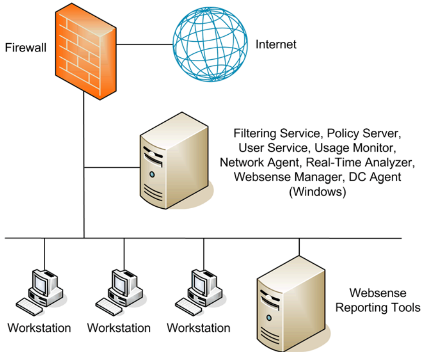
Stand-Alone Deployment in a Windows Environment
